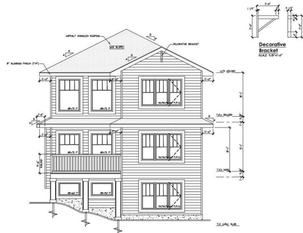
Rear Elevation
